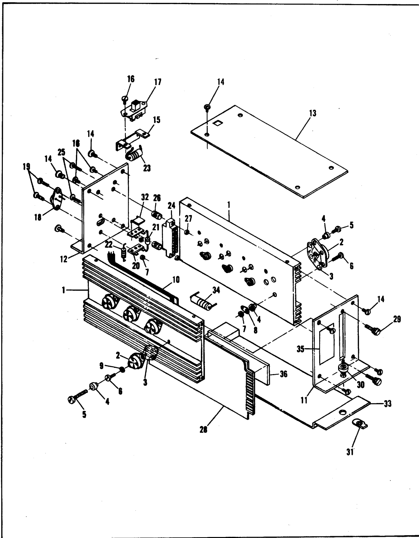
Figure 11-5. 1D395 Amplifier
