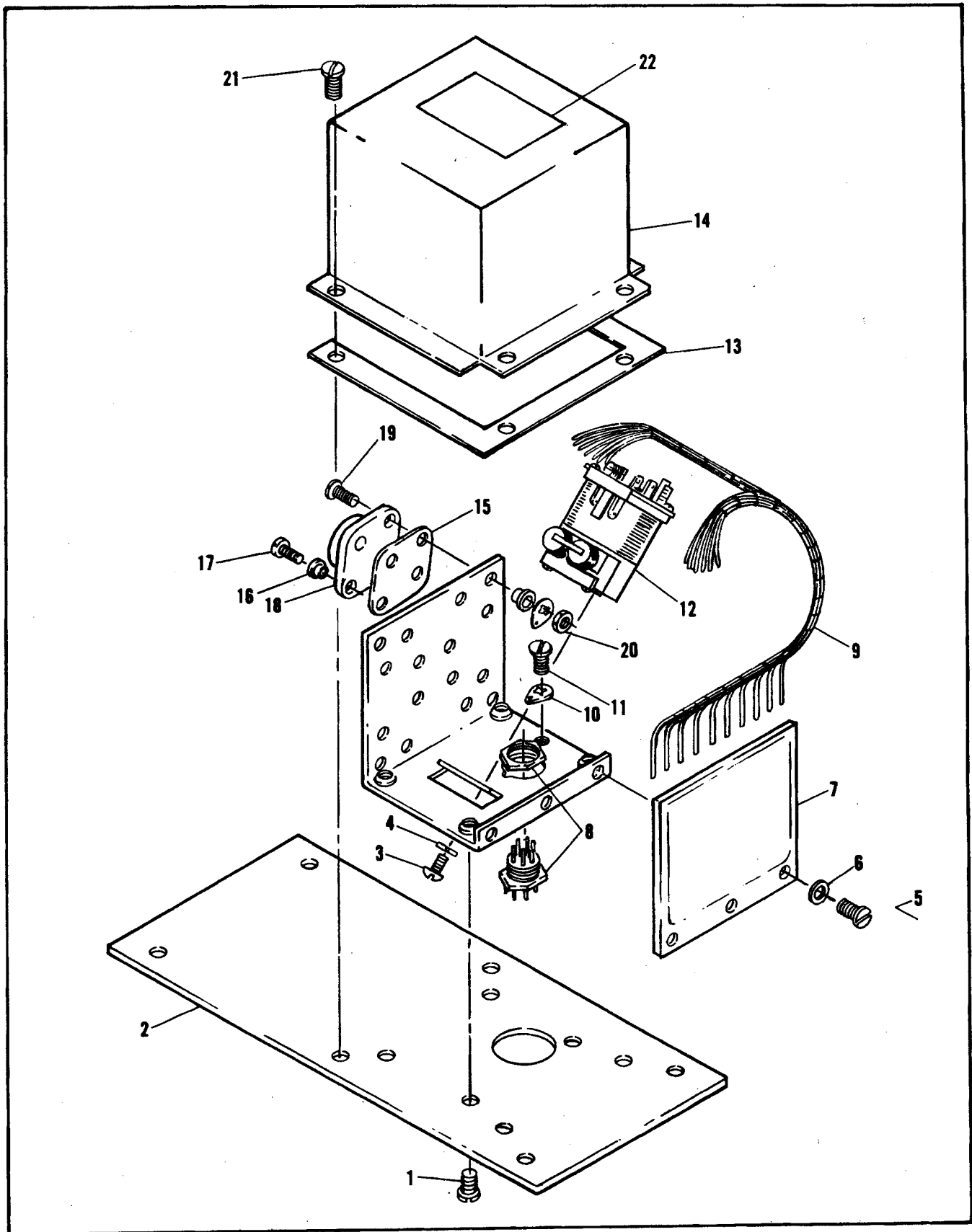
1C359 Gyro-Amplifier
