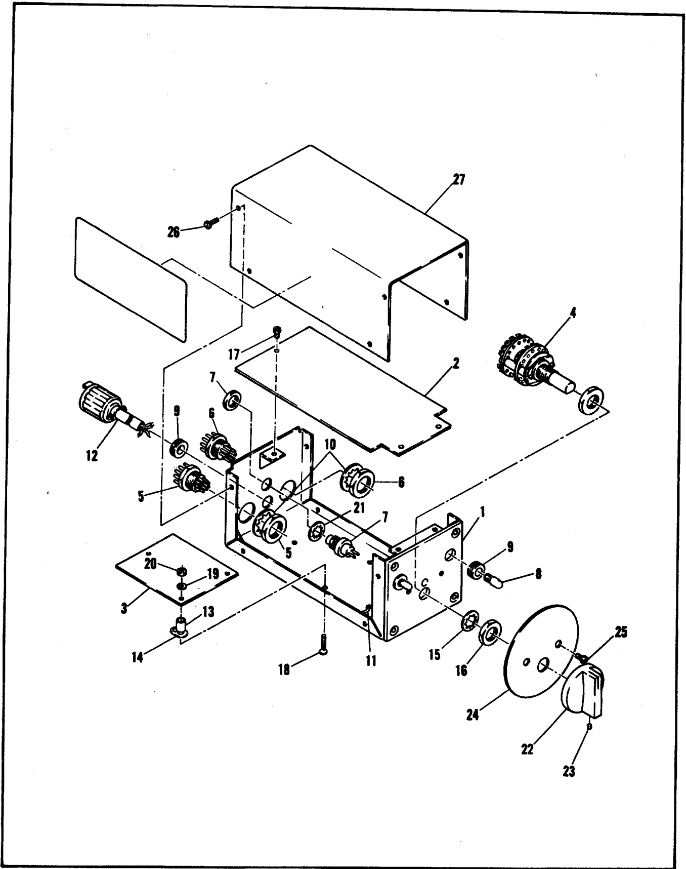
1C388 Radio Coupler
