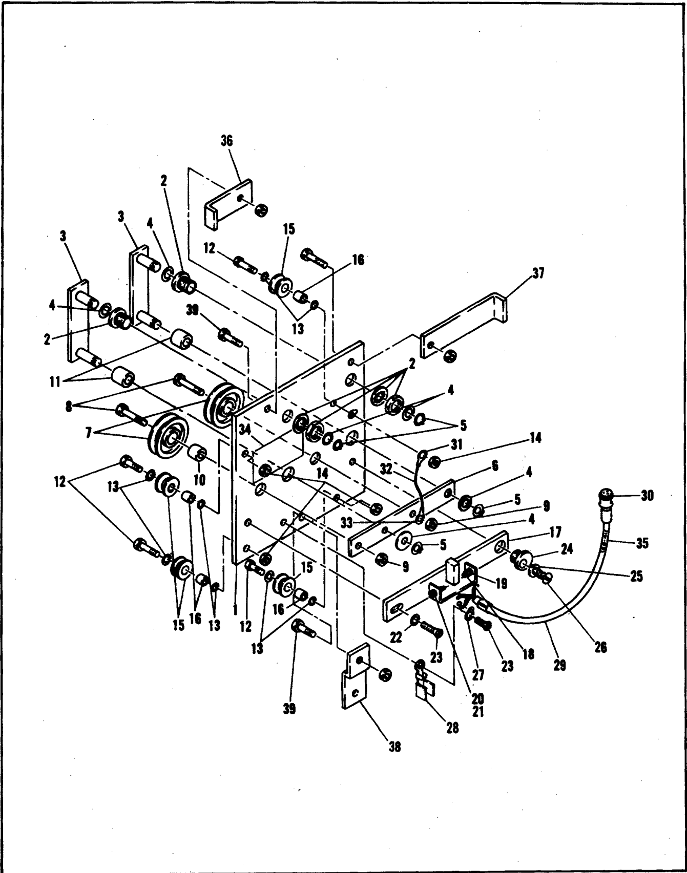
1C377-Trim Sensor Assembly
