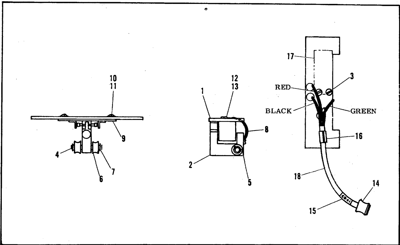
1C318 Pitch Trim Sensor Assembly
