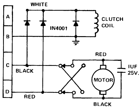
SCHEMATIC - B FOR MANUAL TRIM ONLY
