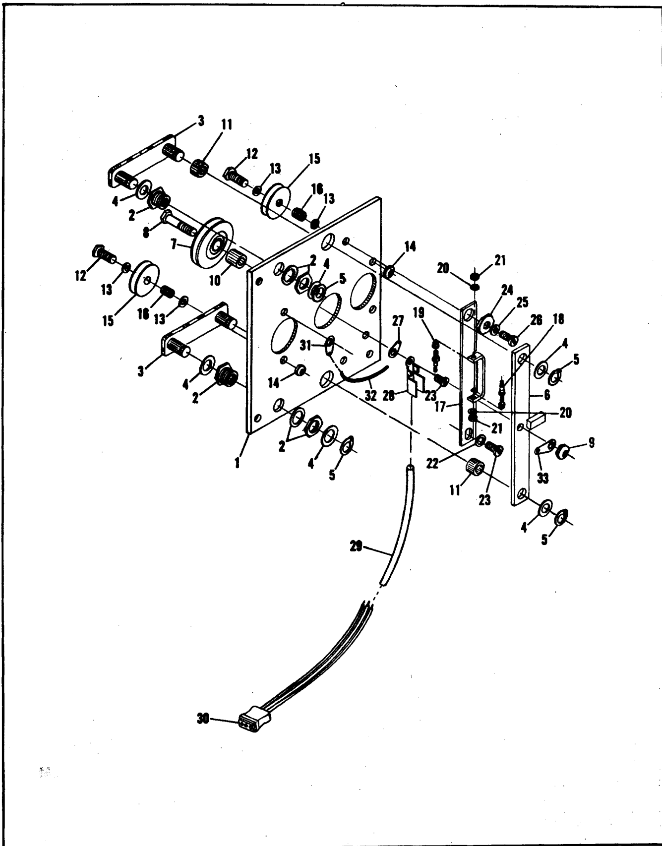
1C365 Trim Sensor Assembly
