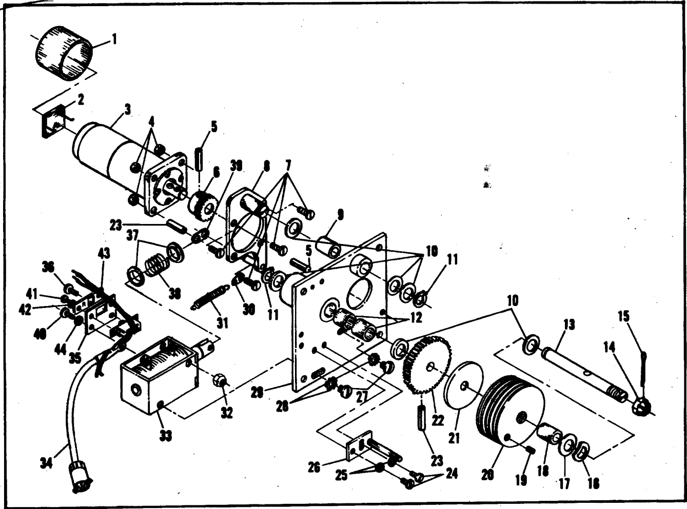
Typical Servo
