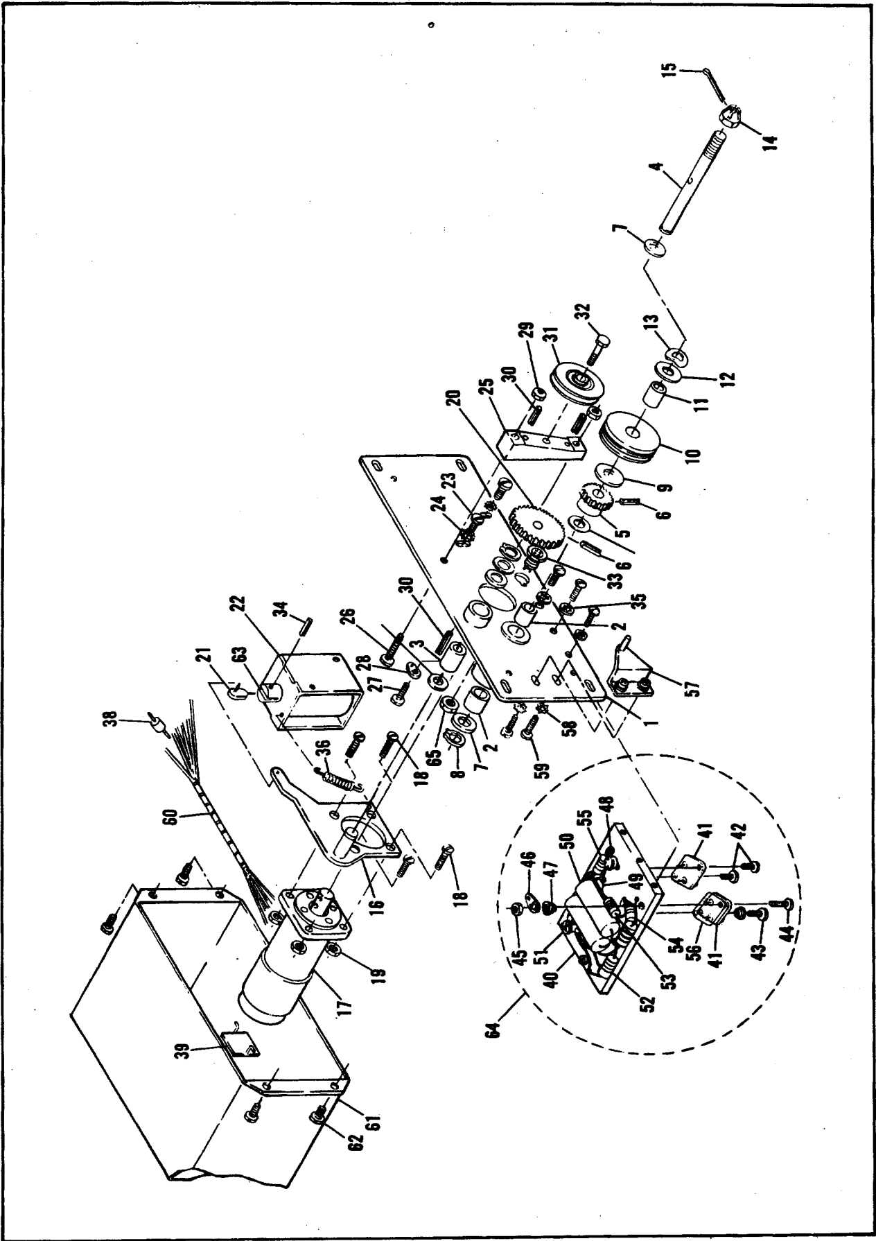
Typical Trim Servo
