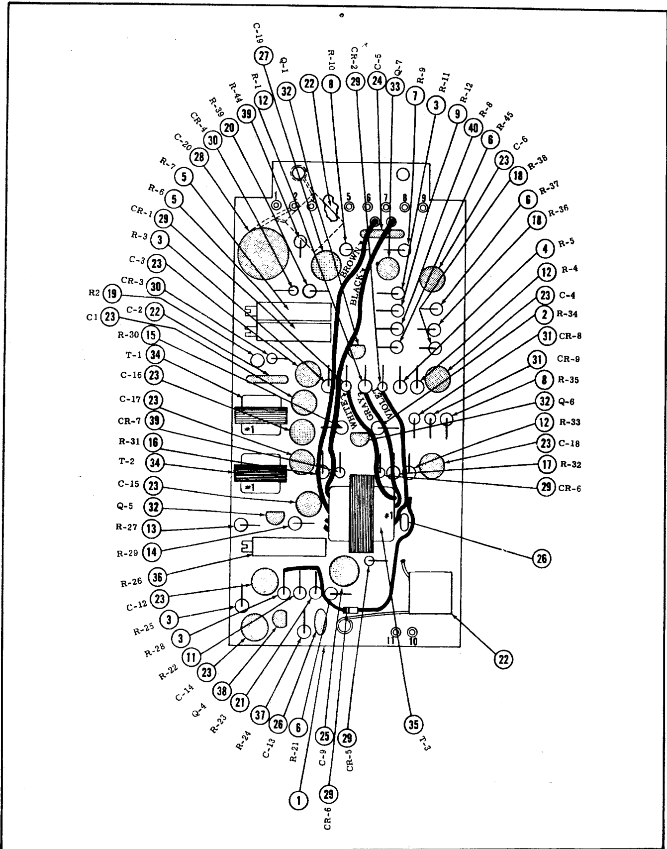
1C412 Radio Coupler Printed Circuit Board
