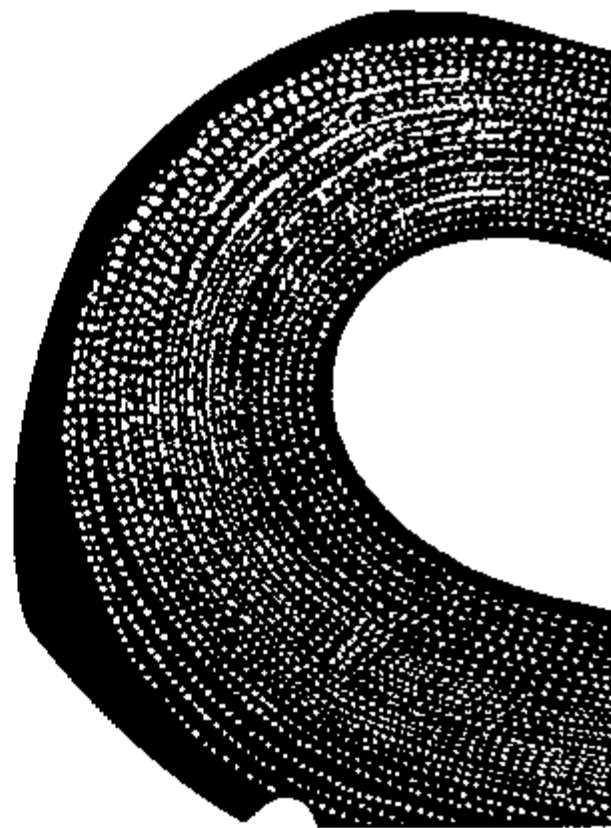
Loaded Cross Section
