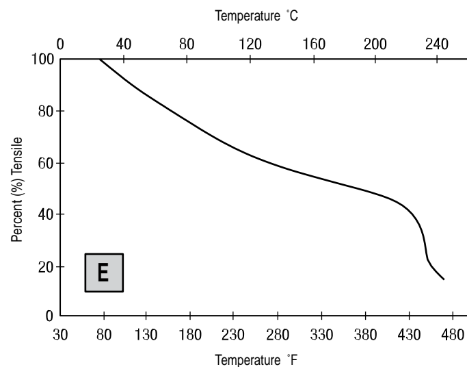
Tensile vs Temperature
