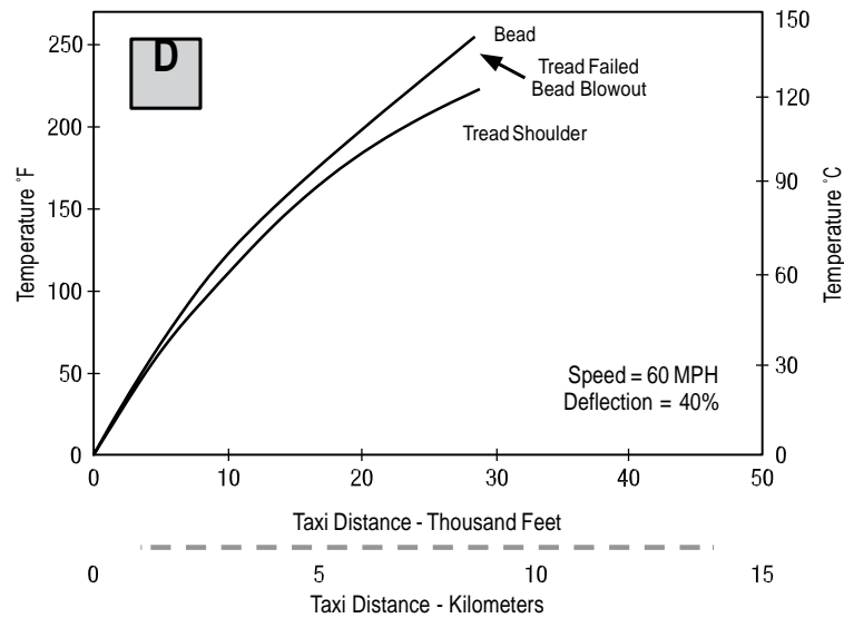
Temperature Rise vs Taxi Distance
