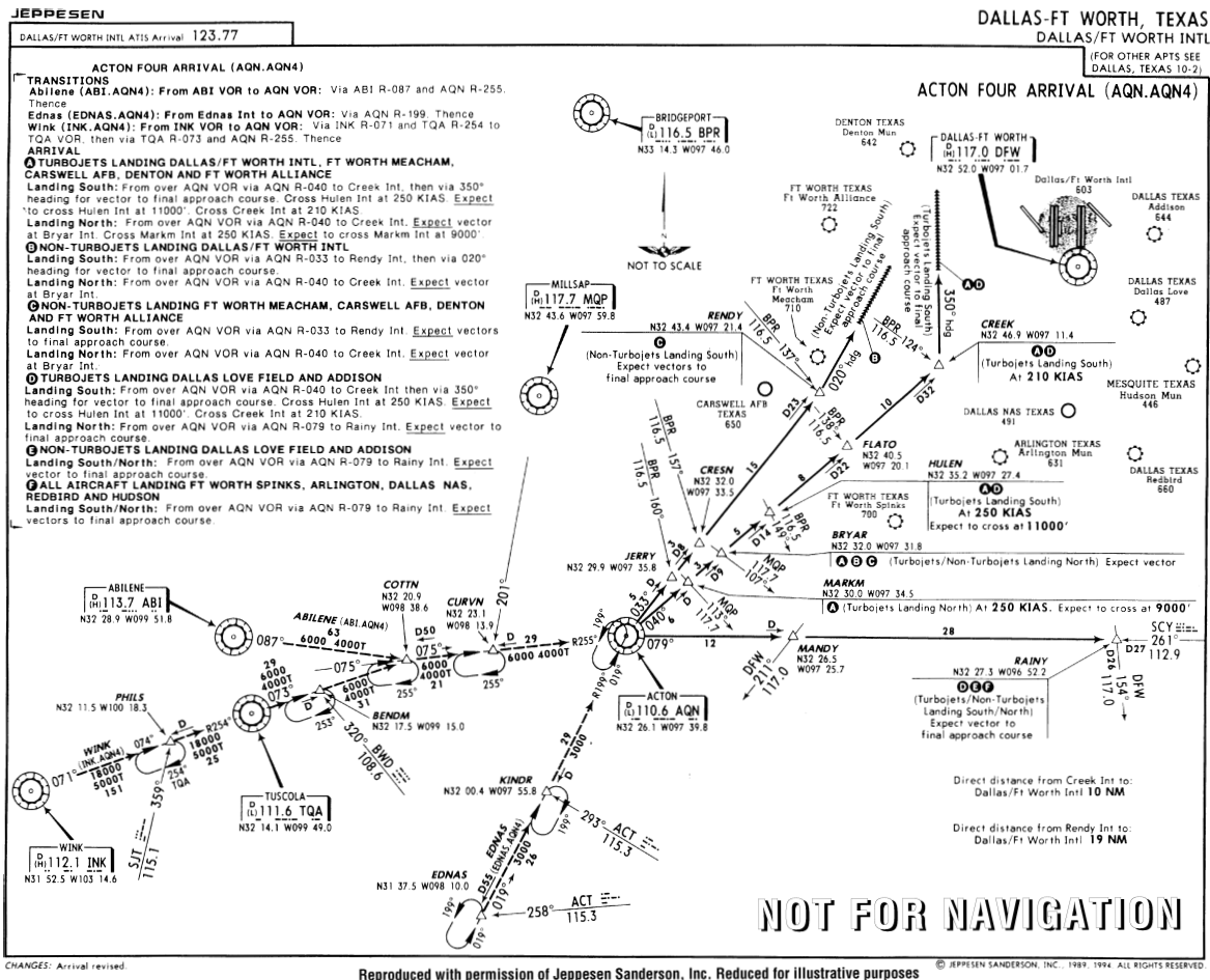
Reproduced with permission of Jeppesen Sanderson, Inc. Reduced for illustrative purposes © JEPPESAN SANDERSON, INC., 1989, 1994. ALL RIGHTS RESERVED. Figure 6-45
